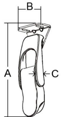
90° Mount
